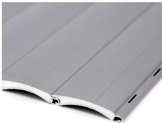
Aluminium-Profil CD 139
