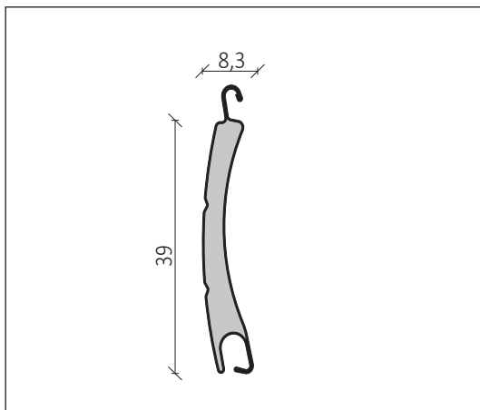
Aluminium-Profil CD 139
