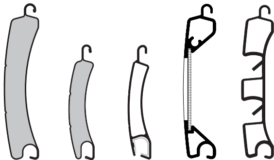
CD 77 19 x 78,5mm CD 200 14 x 55mm CD 70/E 13,2 c 54mm CD 78 18 x 78 mm CD 79/R 18 x 78 mm
